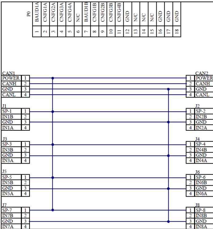
DP-34044-2-XXX I/O Diagram
