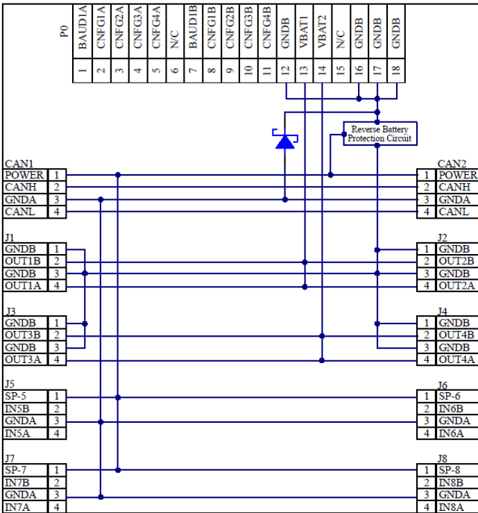
DP-34044-1-XXXX I/O Diagram
