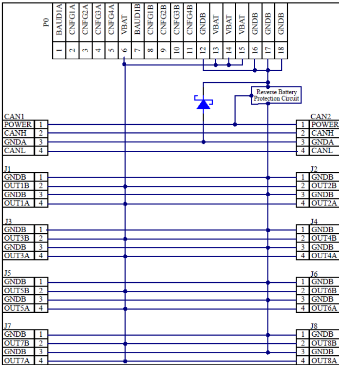
DP-34044-5-XXXX I/O Diagram
