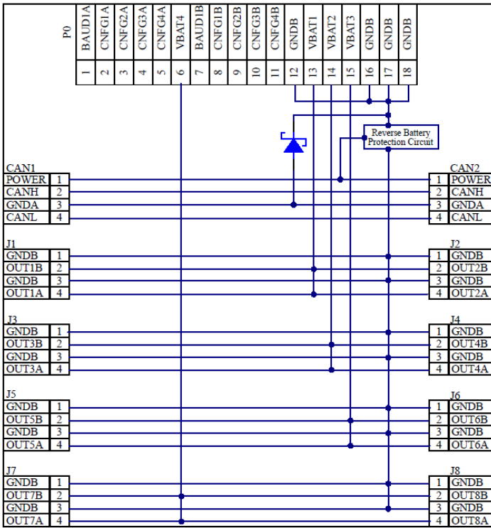
DP-34044-3-XXXX I/O Diagram
