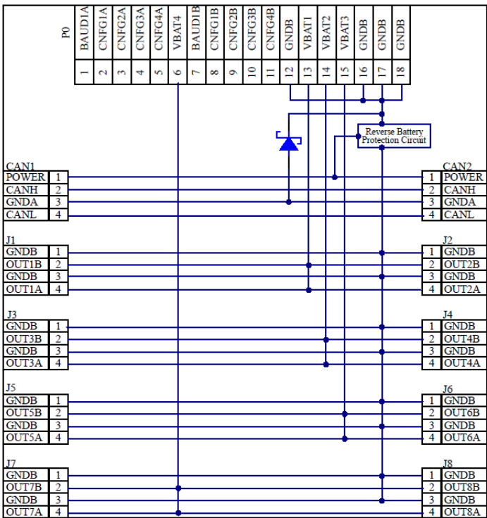
DP-34044-4-XXXX I/O Diagram
